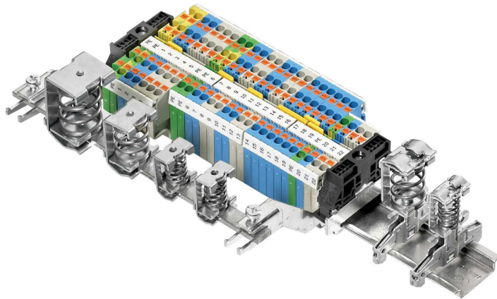
WST Series shielding terminals provide convenient grounding and interference immunity for cables that require grounding shields (WTSSeriesterminals.jpg)
